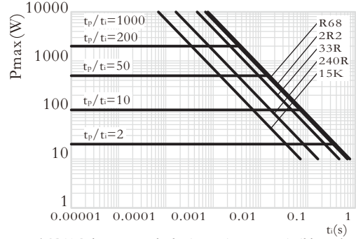
ACR10 Pulse on a regular basis; maximum permissible peak pulse power ( \hat{P}_{max} ) as a function of pulse duration ( t_i )
