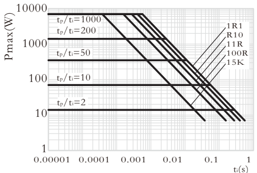
ACR04 Pulse on a regular basis; maximum permissible peak pulse power ( \hat{P}_{max} ) as a function of pulse duration ( t_i )
